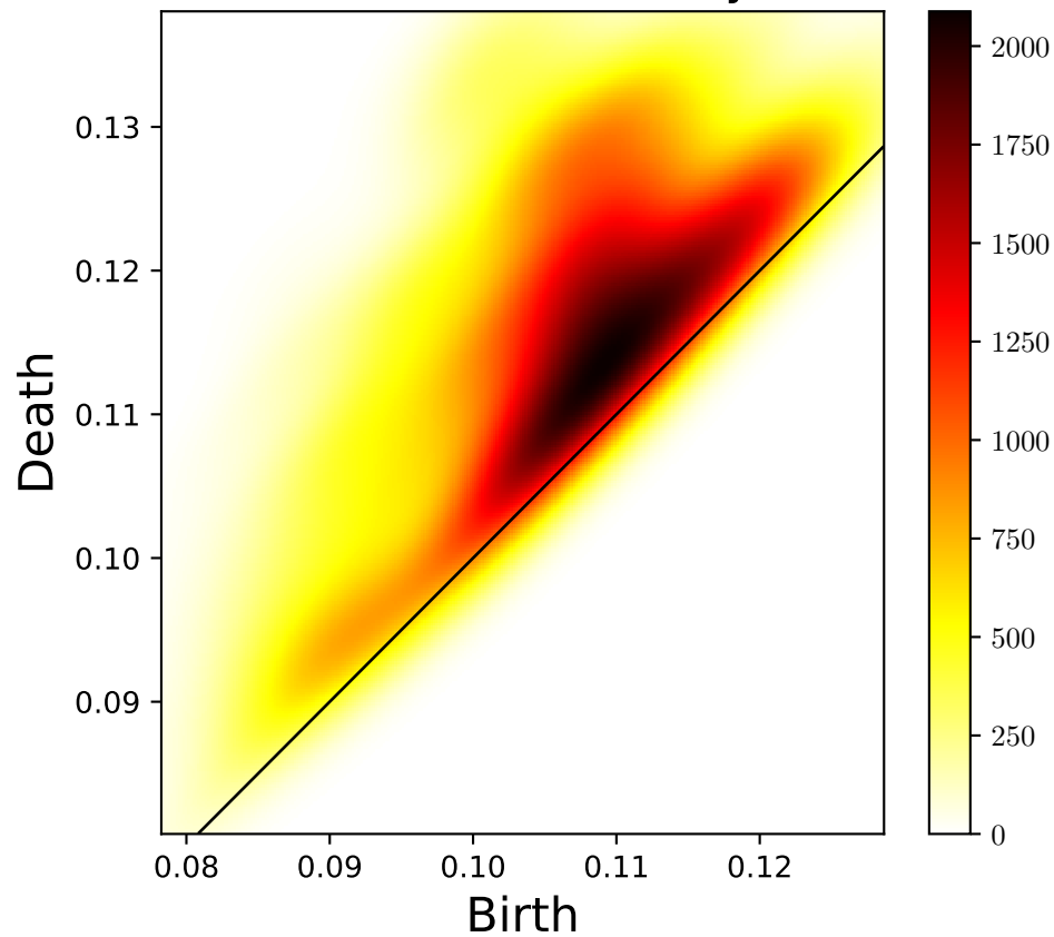
Persistence density
