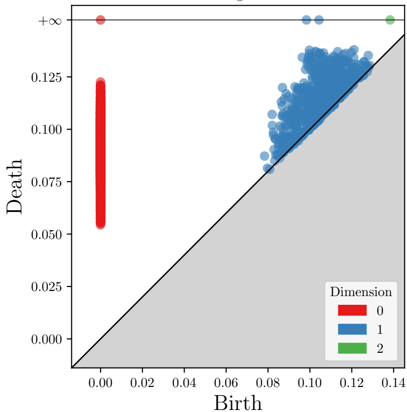
Persistence diagram of a torus
