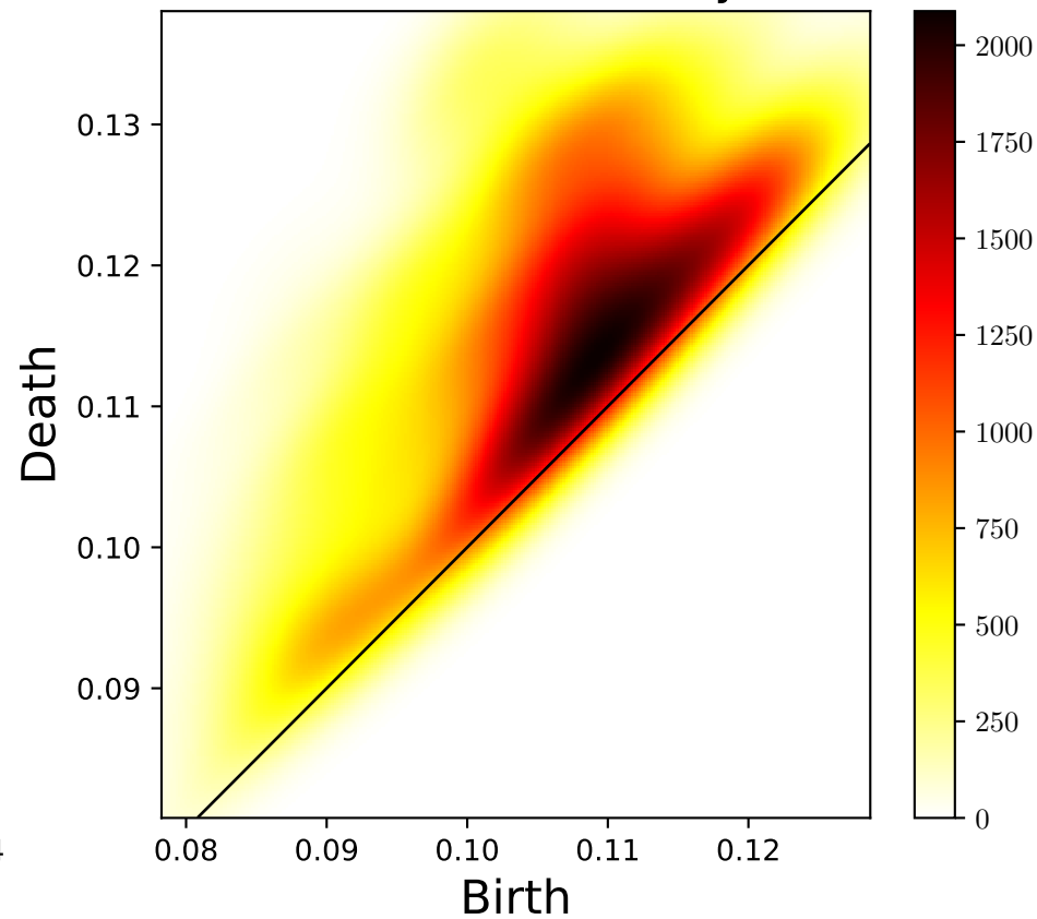
Persistence density
