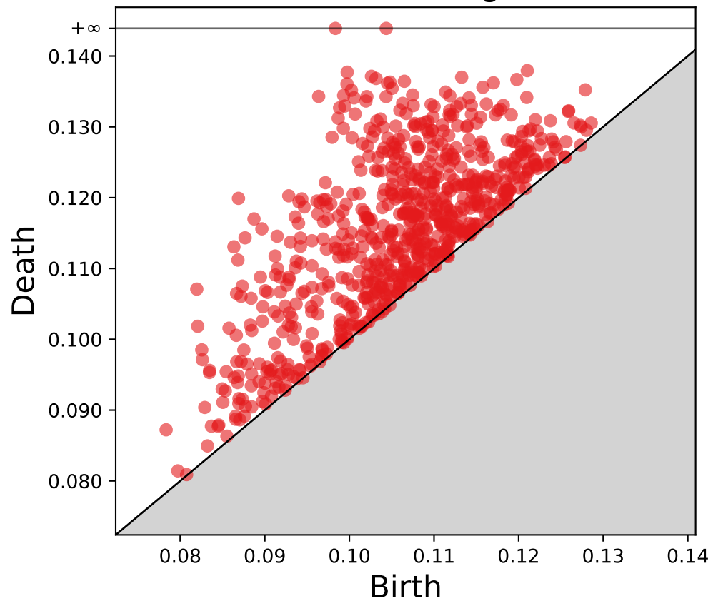
Persistence diagram
