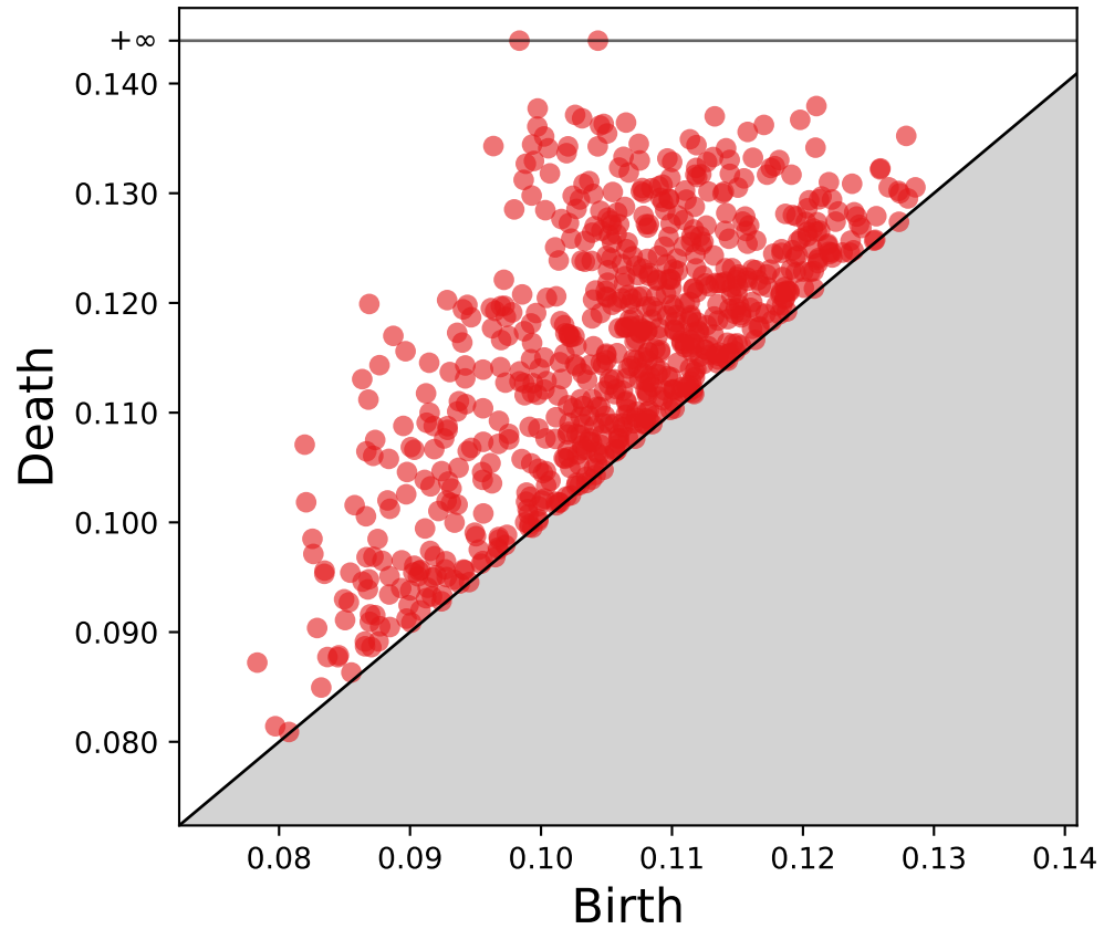
Persistence diagram
