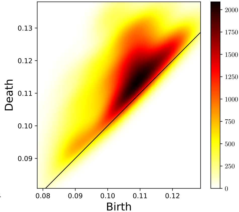
Persistence density
